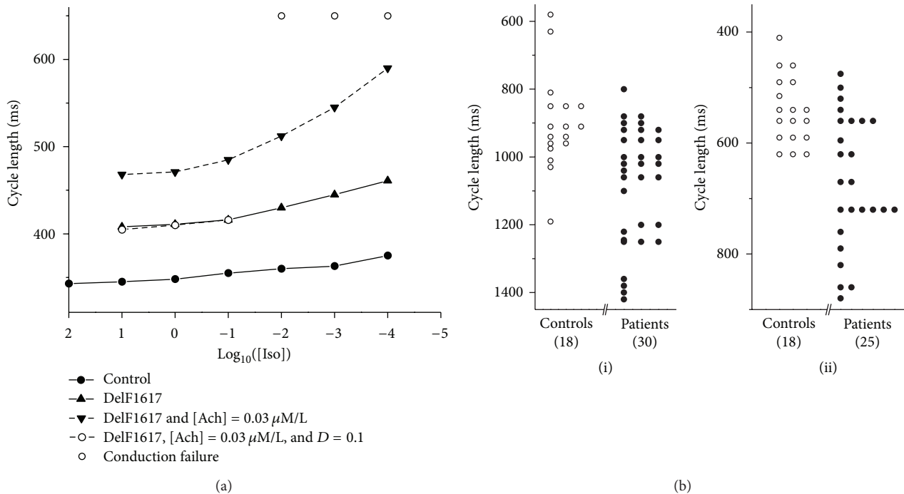
FIGURE 5: (a) Measured pacemaking CL against [Iso] computed from tissue model. Solid circles: controls; solid triangle: DelF1617 mutation; solid inverted triangles: DelF1617 and [\text{Ach}] = 0.03 \mu\text{M/L} ; open circles: DelF1617, [\text{Ach}] = 0.03 \mu\text{M/L} , and D = 0.1 ; solid line: without conduction block; dashed line: conduction block occurs in AS. (b) Distribution of CL in controls and patients (i) before and (ii) after Iso injection. Open circles: clinical data of Vallin and Edhag from controls; solid circles: data of Vallin and Edhag from patients.
