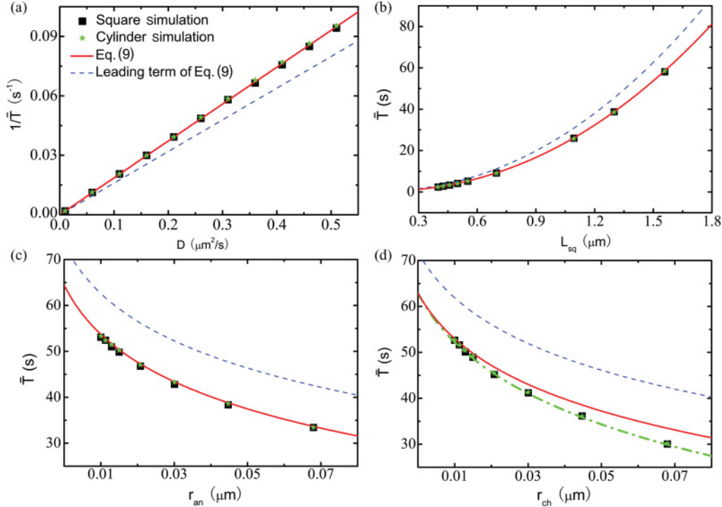
FIG. 3. (Color online) Spatially averaged MFPT for a diffusing IP 3 R channel in a square domain and a square-shaped cylindrical domain. Square symbols, simulation data for the square domain; star symbols, simulation data for square-shaped cylinder with H_{cyl} = \pi R_C = L_{sq} . (a) 1/\bar{T} as a function of D at r_{ch} = 9 nm, r_{an} = 10 nm, and L_{sq} = 1.5 μm; (b) \bar{T} as a function of L_{sq} (or H_{cyl} ) at r_{ch} = 9 nm, r_{an} = 10 nm, and D = 0.1 μm 2 /s; (c) \bar{T} as a function of r_{an} at r_{ch} = 9 nm, D = 0.1 μm 2 /s, and L_{sq} = 1.5 μm; and (d) \bar{T} as a function of r_{ch} at r_{an} = 10 nm, D = 0.1 μm 2 /s, and L_{sq} = 1.5 μm. Red solid lines, theoretical results in Eq. (9) with L = L_{sq} ; blue dashed lines, the leading order term of Eq. (9). The green dashed-dotted line in (d) corresponds to the theoretical result in Eq. (9) with L = L_{sq} - r_{ch} .
