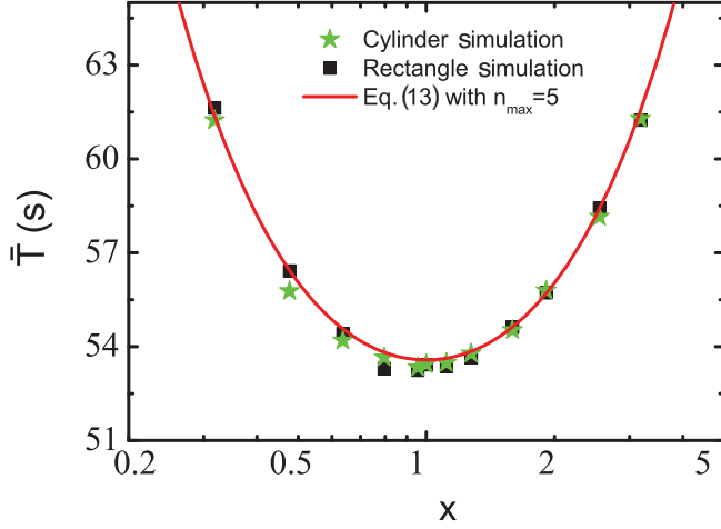
FIG. 5. (Color online) Dependence of the average MFPT on the aspect ratio x = H/\pi R_C of a cylindrical domain (or on the ratio of x = \text{width}/\text{length} for a rectangular domain) with an anchor site ( r_{\text{an}} = 10 nm) at the center. The area of the respective domain is kept fixed at A = 9 \mu\text{m}^2 . Green star symbols, simulation data for the cylindrical domain; black square symbols, simulation data for the rectangular domain. The red curve corresponds to the theoretical result [Eq. (13)] with n_{\text{max}} = 5 , D = 0.1 \mu\text{m}^2/\text{s} , and \varepsilon = 19 nm.
