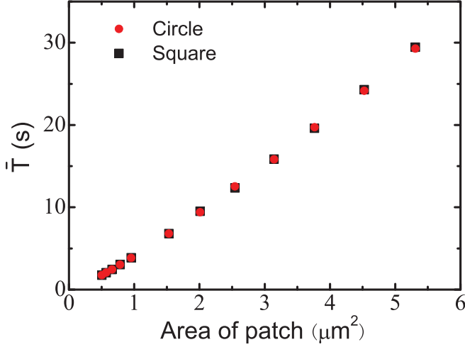
FIG. 4. (Color online) Dependence of the spatially averaged MFPT on the domain area. Red circle symbols, circular domain and black square symbols, square domain. Parameters are r_{\text{ch}} = 9 nm, r_{\text{an}} = 10 nm, and D = 0.1 \mu\text{m}^2/\text{s} .
