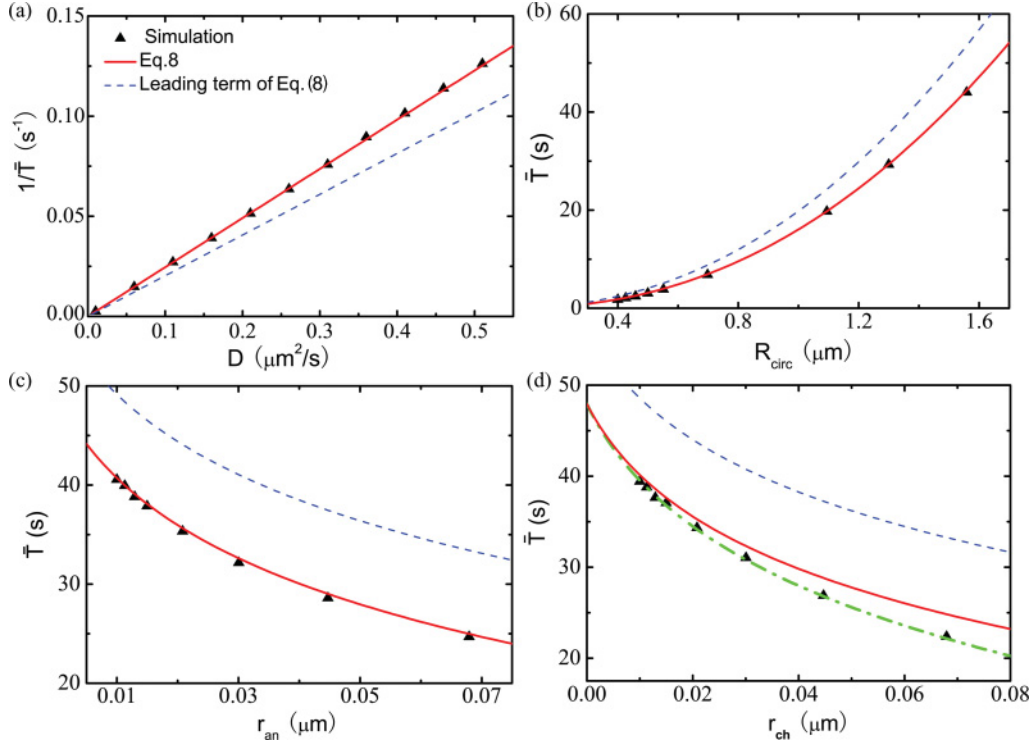
FIG. 2. (Color online) Average MFPT for a diffusing IP 3 R channel in a circular patch with an anchor site of radius r_{\text{an}} at its center. (a) 1/\bar{T} as a function of D at r_{\text{ch}} = 9 nm, r_{\text{an}} = 10 nm, and R_{\text{circ}} = 1.5 \mu\text{m} ; (b) \bar{T} as a function of R_{\text{circ}} at r_{\text{ch}} = 9 nm, r_{\text{an}} = 10 nm, and D = 0.1 \mu\text{m}^2/\text{s} ; (c) \bar{T} as a function of r_{\text{an}} at R_{\text{circ}} = 1.5 \mu\text{m} , r_{\text{ch}} = 9 nm, and D = 0.1 \mu\text{m}^2/\text{s} ; (d) \bar{T} as a function of r_{\text{ch}} at R_{\text{circ}} = 1.5 \mu\text{m} , r_{\text{an}} = 10 nm, and D = 0.1 \mu\text{m}^2/\text{s} . Black symbols, stochastic simulation data; red solid lines, theoretical results in Eq. (8) with R = R_{\text{circ}} ; blue dashed lines, the leading order term of Eq. (8). The green dashed-dotted line in (d) denotes the theoretical result in Eq. (8) with R = R_{\text{circ}} - r_{\text{ch}} .
