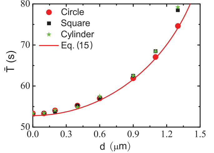
FIG. 6. (Color online) Dependence of the average MFPT on the distance d of the anchor site from the patch center for different domain shapes. Red circles, simulation data for the circular patch with R = 1.69 \mu\text{m} ; black squares, simulation data for the square patch (all boundaries reflecting) with L_{\text{sq}} = 1.5 \mu\text{m} ; green stars, simulation data for the cylindrical patch with L_{\text{cyl}} = 1.5 \mu\text{m} = \pi R_C . The red curve corresponds to the theoretical result in Eq. (15). Here, r_{\text{ch}} = 9 nm, r_{\text{an}} = 10 nm, and D = 0.1 \mu\text{m}^2/\text{s} .
