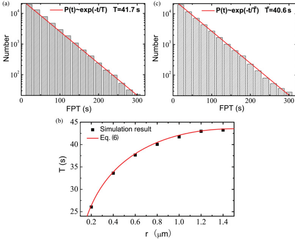
FIG. 1. (Color online) The FPT for a Brownian IP 3 R channel in a circular patch with an anchor site at its center. (a) Exponential distribution of the FPT for a channel starting at a given distance r = 1 \mu\text{m} . (b) The MFPT as a function of the distance r . Black squares, stochastic simulation data; red solid line, the theoretical result in Eq. (6) with R = R_{\text{circ}} . (c) Exponential distribution of the FPT for a channel starting at arbitrary positions in the patch. Parameters are r_{\text{an}} = 10 nm, r_{\text{ch}} = 9 nm, R_{\text{circ}} = 1.5 \mu\text{m} , and D = 0.1 \mu\text{m}^2/\text{s} . The distribution can be fitted by a straight line with a slope of 40.6 s.
